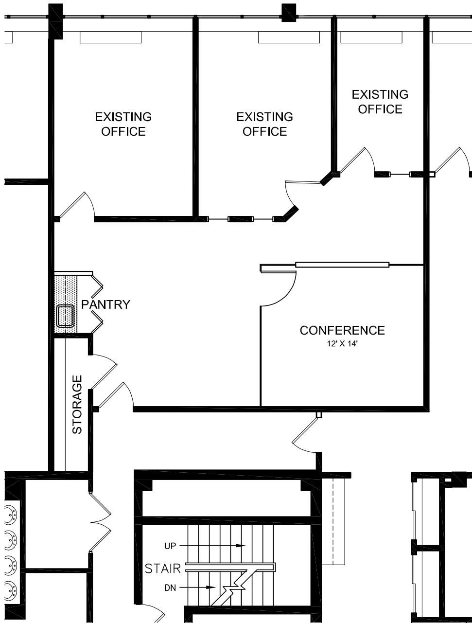
1 SCHEMATIC PLAN 1/8" = 1'-0"
